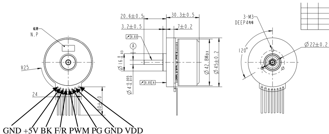
FIG. 1 Mechanical dimensions
